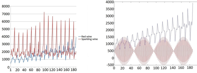
Figure 5. Red wine vs sparkling wine and generated series, 1980–1994.
