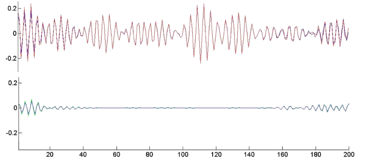
Figure 1. Reconstructions differences for the model (23) with perturbation \sigma\varepsilon_n \sim N(0, 0.25) : \tilde{x}^{(1)} - \tilde{x}^{(3)} , \tilde{x}^{(2)} - \tilde{x}^{(4)} (top); \tilde{x}^{(2)} - \tilde{x}^{(4)} , \tilde{x}^{(2)} - \tilde{x}^{(3)} (bottom).
