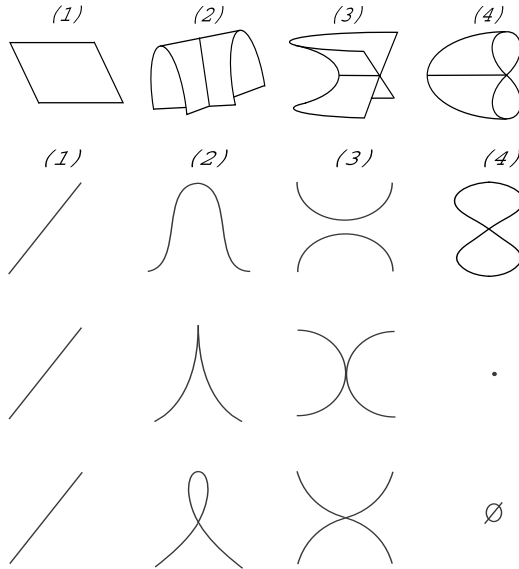
FIGURE 1. Typical isotropic bifurcations
