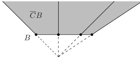
FIGURE 18. The truncated cone.
