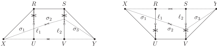
FIGURE 13. Two of the pairs of jagged paths contributing to XY are drawn in each chart. Contrary to appearances, none of the eight jagged paths appearing here bend!
