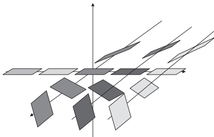
FIGURE 3. A contact structure.
