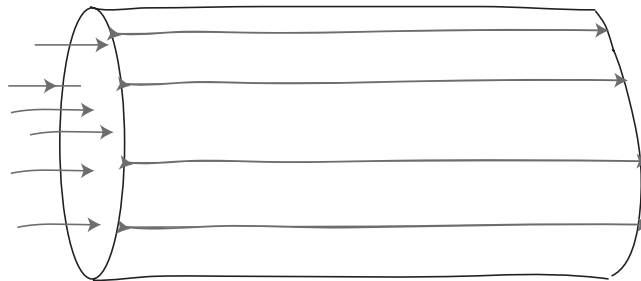
FIGURE 1. A flow tube with a flow being standard at the boundary.
