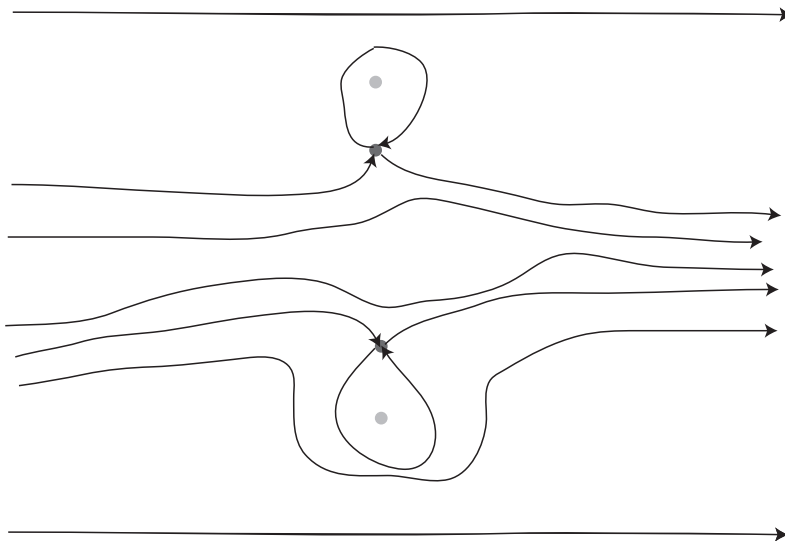
FIGURE 2. Two periodic orbits are introduced in order to have a flow without rest points, but not all flow lines entering left leave on the right.
