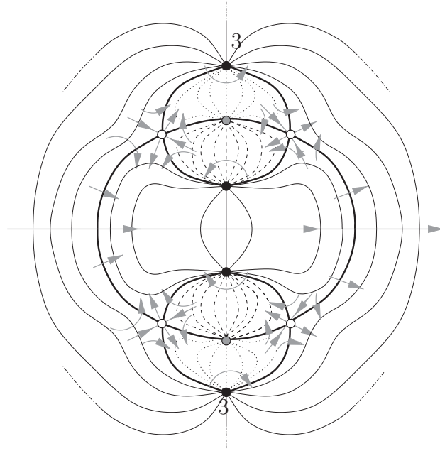
FIGURE 8. A second example, illustrating a finite energy foliation associated to S^3 . The grey dots represent a periodic orbit of index 1, the white dots periodic orbits of index 2 and the black dots periodic orbits of index 3. The leaves are again disk-like and annuli-like surfaces. The rigid surfaces are represented by bold curves. Dotted and dashed surfaces represent families of annuli-like surfaces connecting periodic orbits of index 3 with periodic orbits of index 1. Thin curves represent disk-like surfaces asymptotic to periodic orbits with index 3. The grey arrows picture the flow of the Reeb vector field.
