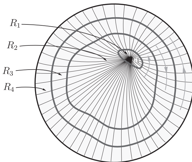
FIGURE 20. A limiting foliation for the integrable disk map \psi_H from Figure 18. The leaves with vanishing d\lambda -energy correspond to the quasi-periodic orbits in the invariant circles which have the chosen rotation number \omega and which surround the chosen elliptic fixed point e_1 . Each leaf with non-zero d\lambda -energy is a strip connecting two such orbits on neighboring circles. The flow is transverse to these strips in alternating directions as one passes through a circle, as indicated by the grey arrows.
