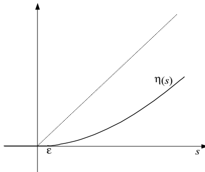
FIGURE 13. A function \eta(s)
