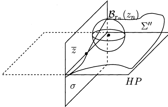
FIGURE 10. If we rescale B_{r_n}(z_n) , then we find a sequence of stable minimal surfaces \Sigma^n which converge to the half-plane HP .
