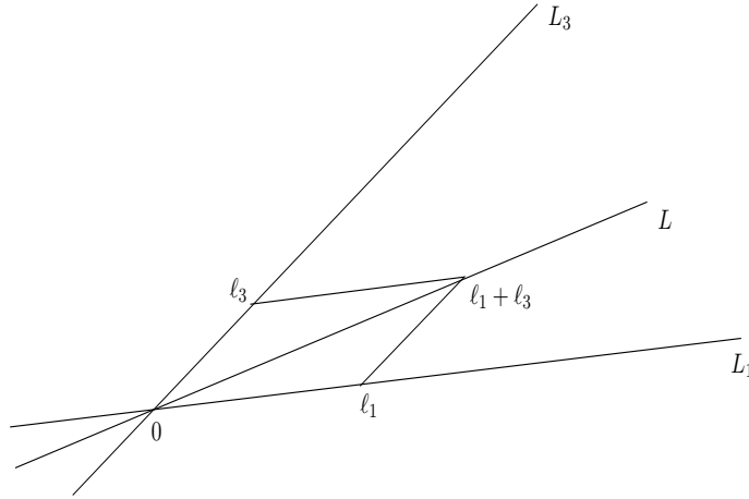
FIGURE 2. Let L_1 and L be transverse to L_3 . Then the vector \ell_3 \in L_3 is the image of the vector \ell_1 \in L_1 under the isomorphism T_{13} : L_1 \rightarrow L_3 defined by L . The value at \ell_1 of the quadratic form Q_L^{L_1, L_3} on L_1 based at L_3 and induced by L measures the signed area of the parallelogram with vertices 0, \ell_1, \ell_1 + \ell_3, \ell_3 . Moreover, if also L_1 and L are transverse, then Q_L^{L_1, L_3}(\ell_1) = -Q_L^{L_3, L_1}(\ell_3) , where \ell_1 and \ell_3 are related as above.
