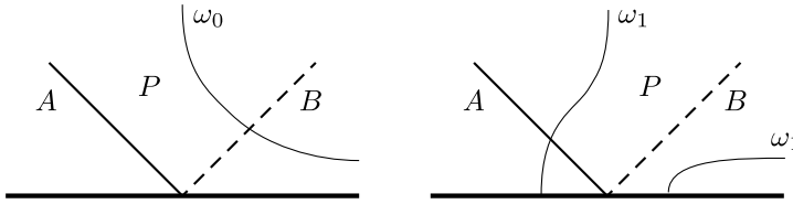
Figure 2: Changing \omega_0 near a corner of P
