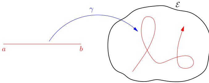
FIGURE 1. The picture we envision is that of “driving” the system along a curve \gamma in \mathcal{E} and losing memory of past density distributions at variable rates depending on local characteristics. That, we submit, is the true nature of memory loss in dynamical systems with slowly varying parameters .
