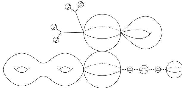
FIGURE 1. A generalized cactoid.
