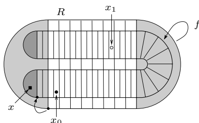
FIGURE 2. The horseshoe map.
