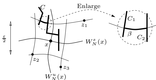
FIGURE 4. An inaccessible point and a nearby continuum.
