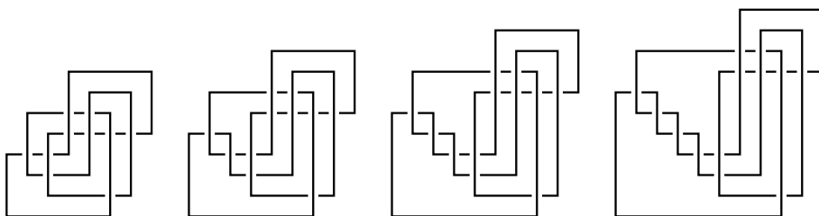
Figure 5: A family of Legendrian pretzel knots.
