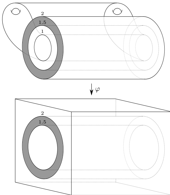
Figure 2: Top, a schematic of Z , with the region A shown in gray. Bottom, a schematic of (Y \times I) \setminus \varphi((S^1 \times D_{1.5}^2) \times I) , with \varphi(A) shown in gray.
