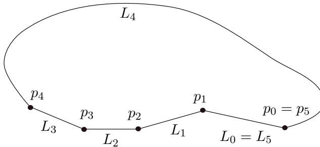
Figure 3: A 5-gon.
