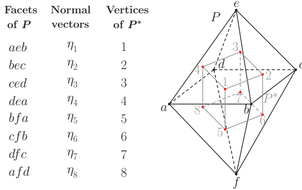
Figure 1: Polar duality for the octahedron and the cube.
