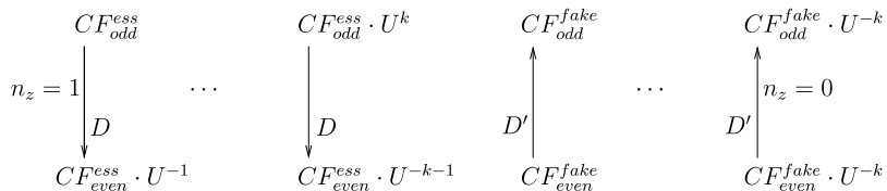
Figure 3. The chain complex of CF^+(Y) .
