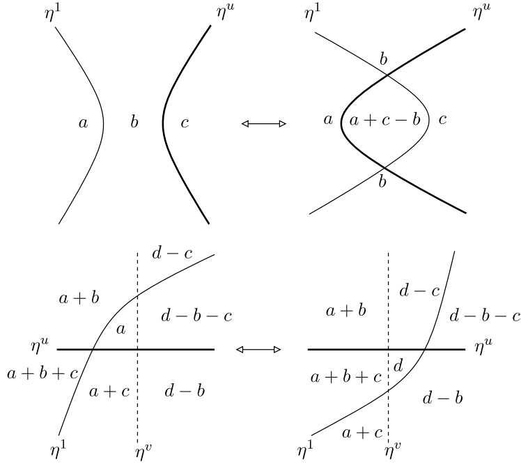
Figure 2. Local coefficients of D and \tilde{D} .
