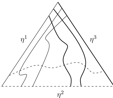
Figure 4. Induced tiling on \Delta_i .
