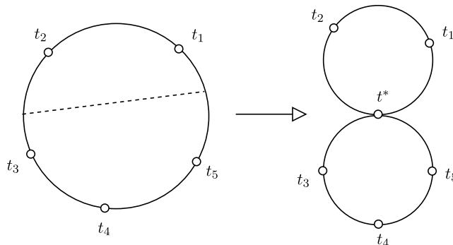
Figure 1. The map that induces the addition operation on the Whitney n -gons.
