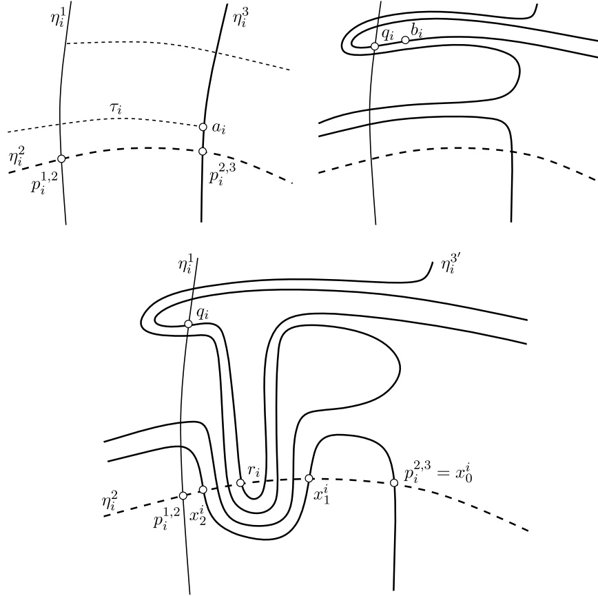
Figure 3. The isotopy of the \eta^3 circles in U_i .
