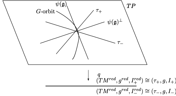
Figure 3. For the generalized Kähler quotient, there are two Riemannian models for TM^{\text{red}} given by spaces \tau_{\pm} transversal to the G -orbit. Each of \tau_{\pm} induces a complex structure on TM^{\text{red}} making it into a bihermitian manifold.
