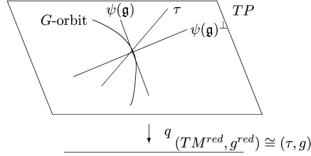
Figure 2. The metric induced on TM^{\text{red}} is modeled on a space transversal to the G -orbits but not necessarily orthogonal to them.
