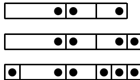
Figure 10: The bijection of Proposition 3.13 where (4_4, 2_1, 2_2) \in B(8) corresponds to (1_1, 3_3, 2_1, 1_1, 1_1, 1_1) \in A(9) .
