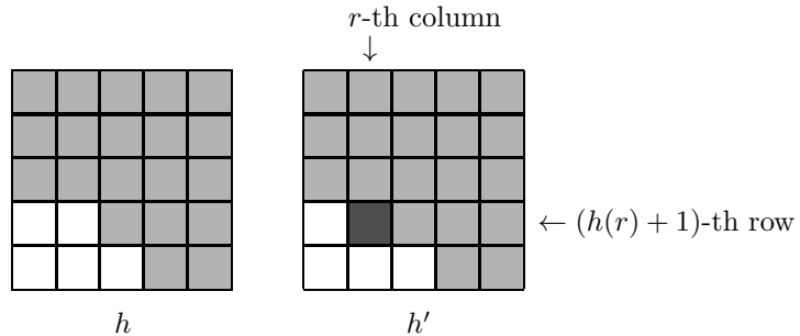
Figure 4: The pictures of h and h' .
