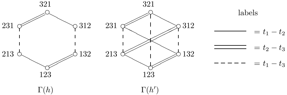
Figure 2: The GKM graphs \Gamma(h) and \Gamma(h') .
