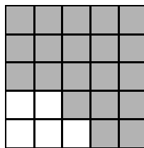
Figure 1: The configuration corresponding to h = (3, 3, 4, 5, 5) .
