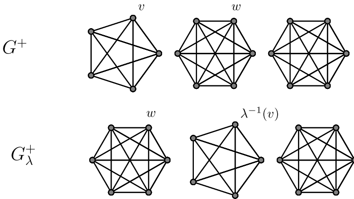
Figure 3: The supercards G^+ and G_\lambda^+ from Lemma 6.1 when p = 5 .
