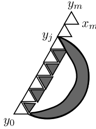
Figure 3: A simple ladder with edges forced by Claim 2.3.
