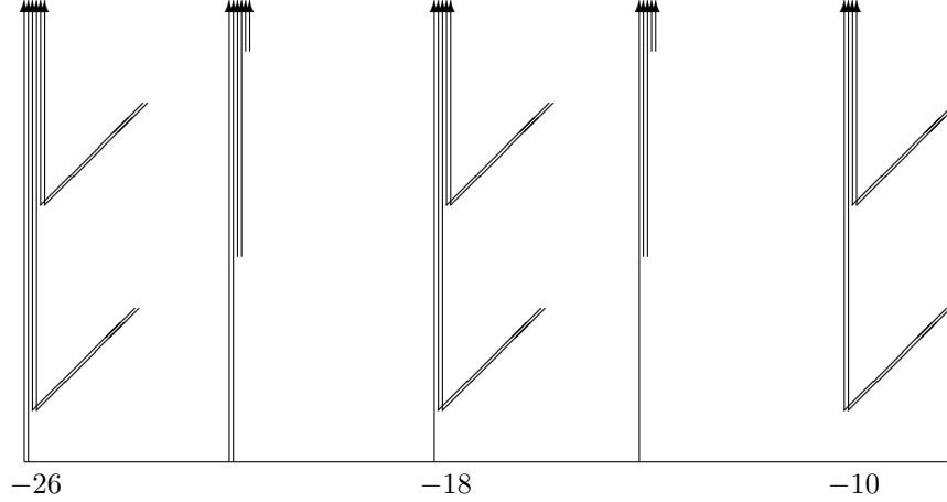
Diagram 3.14. Illustration of Proposition 3.11:
