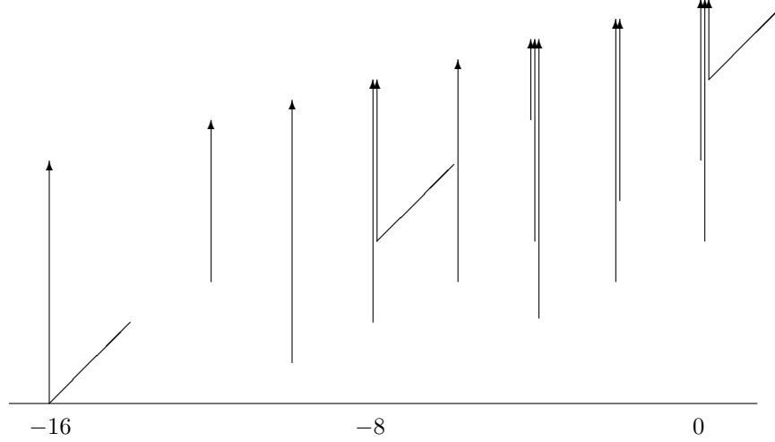
Diagram 5.12. Diagram 5.10 after differentials and filtration shift:
