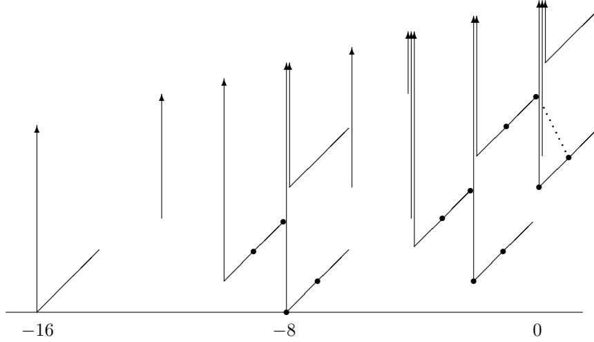
Diagram 5.10. A portion of E_2 for [\Sigma^*CP^\infty, \mathrm{tmf}] :
