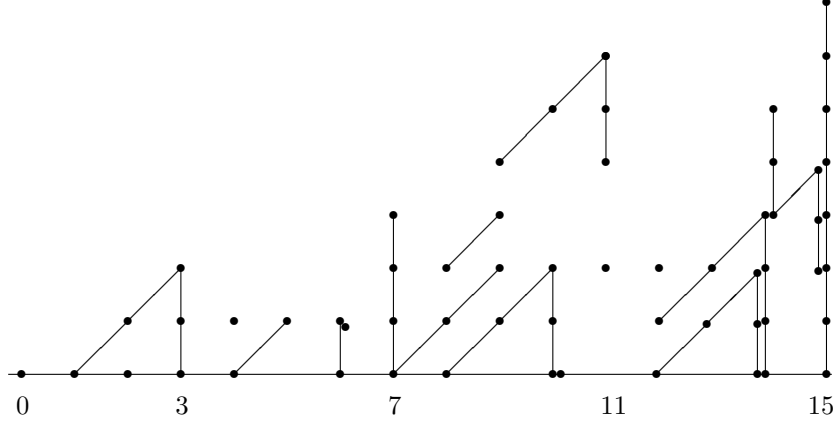
Diagram 2.1. E_2(\mathrm{tmf}_*(P_{-3} \wedge P_3)), * \leq 15 :
