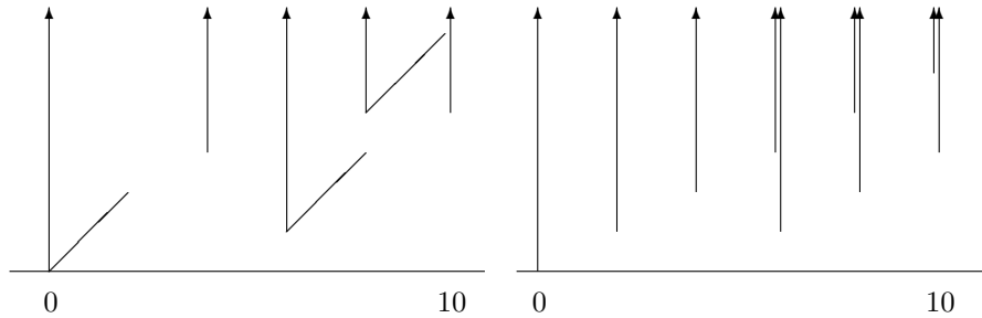
Diagram 5.9. Structure on two types of generators:
