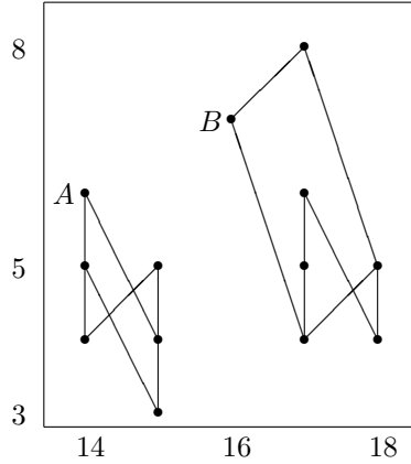
Diagram 5.15. Portion of ASS of \mathrm{tmf} :
