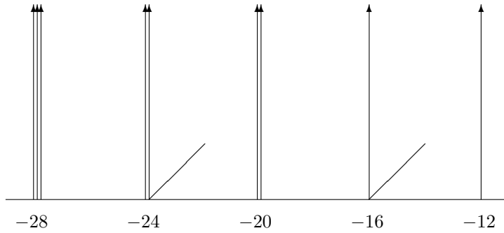
Diagram 5.9. Structure on two types of generators:
