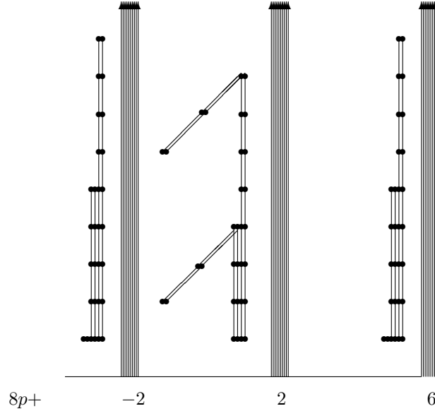
Diagram 3.12. Portion of \mathbf{A} + \mathbf{B} + \mathbf{C} :
