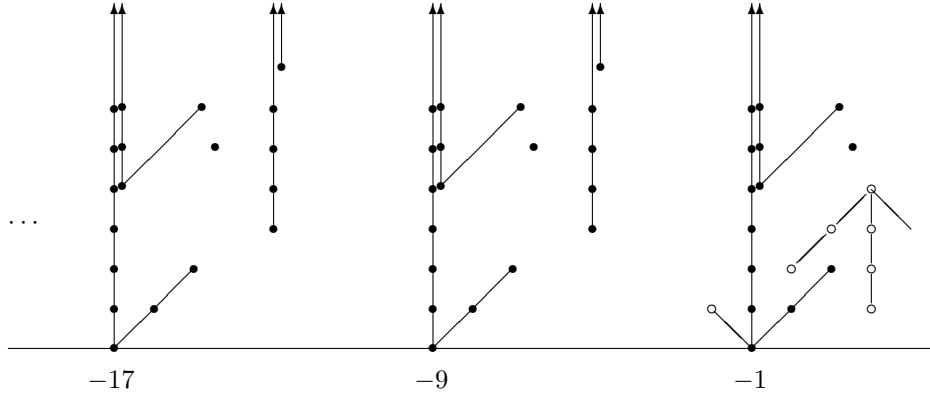
Diagram 3.3. \text{tmf}_*(P_{-\infty}^{-2}), -17 \leq * \leq 2 :
