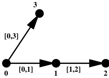
Figure 4: 1-dimensional branching
