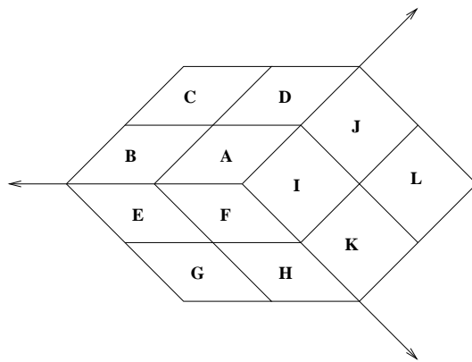
Figure 4: 1-dimensional branching
