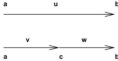
Figure 3: Simplest example of T-homotopy equivalence
