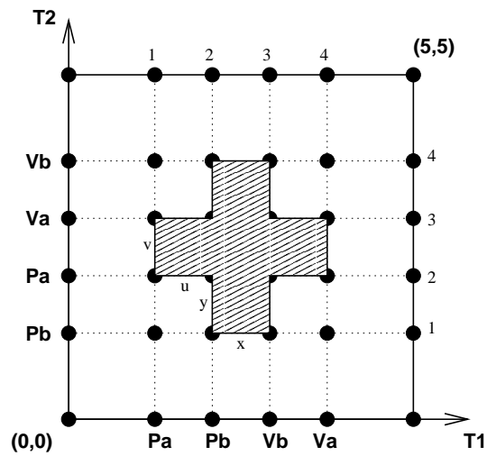
Figure 5: 2-dimensional branching
