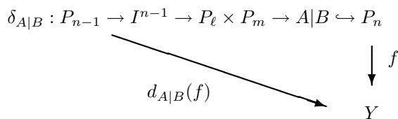
Figure 5: The singular face operator associated with A|B .
