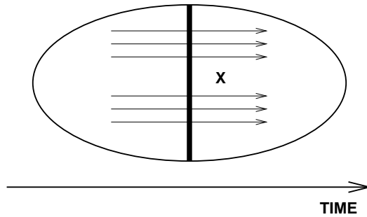
Figure 2: Symbolic representation of \text{Glob}(X) for some topological space X
