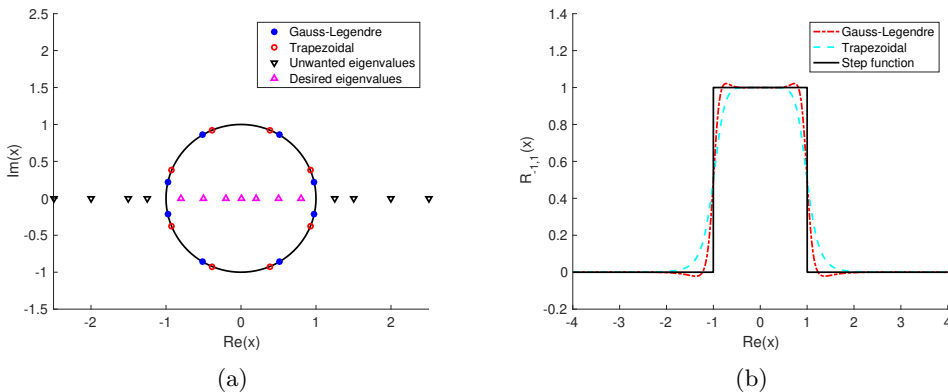
Fig. 1.1: (a) An example of a unit circle contour \Gamma centered at the origin, i.e., the desired spectrum range is (-1, 1) , together with eight Gauss-Legendre quadrature points (solid blue circle) and eight Trapezoidal quadrature points (red circle). The desired eigenvalues (pink up triangular) are inside the contour whereas the unwanted eigenvalues (black down triangular) are outside. (b) A rectangular function in solid black line with rational functions corresponding to the quadratures from (a).
