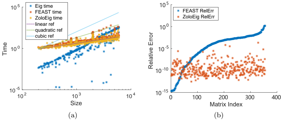
Fig. 3.3: Running time and relative error for matrices in Florida matrix collection solved via ZoloEig and FEAST. The relative error here is the relative error of eigenvalues defined in (3.1).
