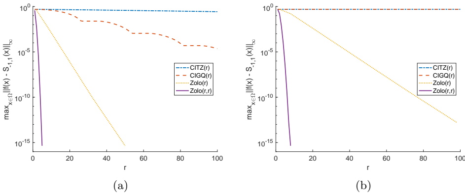
Fig. 2.2: This figure shows the approximation error against degree r for various rational functions as an approximation of the rectangular function supported on (-1,1) . The eigengaps around -1 and 1 are set to be 10^{-2} in (a) and 10^{-6} in (b). The approximation errors of Zolo(r,r) decay significantly faster than other methods. In (b), the line for CITZ is overwritten by that of CIGQ .
