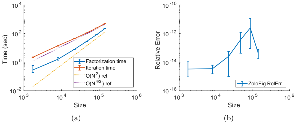
Fig. 3.2: The running time and the relative error for 3D Hamiltonian operator with Gaussian wells solved via ZoloEig. The relative error here is the relative error of eigenpairs defined in (3.1).
