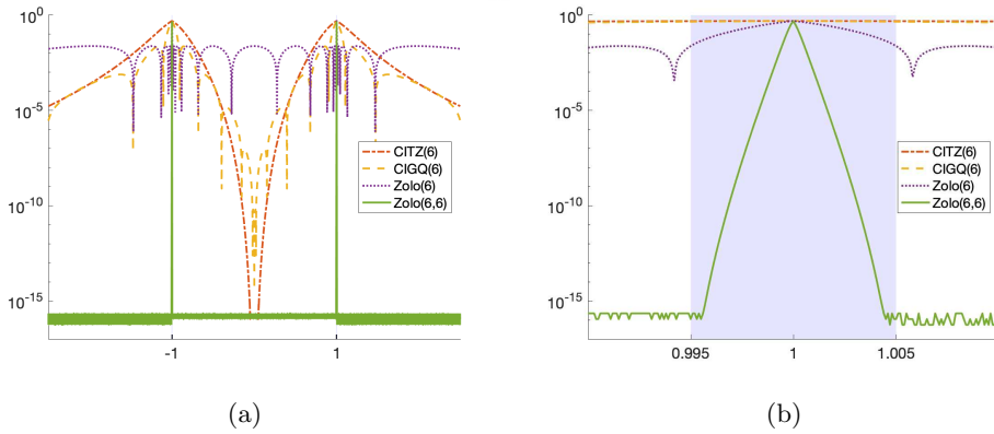
Fig. 2.1: This figure shows the approximation error of various rational filters as an approximation of the rectangular function supported on (-1,1) . The eigengaps around 1 and -1 are set to be 10^{-2} . These functions include: the trapezoidal filter [28, 34] (denoted as CITZ(r) , where r is the number of poles), the Gauss-Legendre filter [22] (denoted as CIGQ(r) , where r is the number of poles), the Zolotarev approximation (denoted as Zolo(r) , where r is the degree), and the proposed Zolotarev filter via compositions (denoted as Zolo(r,r) , where r is the degree). (a) shows the approximation on [-2.5, 2.5] and (b) zooms in on [0.99, 1.01] . Light purple areas are the buffer areas in which it is not necessary to consider the approximation accuracy because of the eigengaps.
