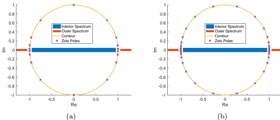
Fig. 2.3: The corresponding contour integral discretization of Zolotarev's function composed with Möbius transformation. The eigengaps here are (-1.1, -0.9) and (0.9, 1.1) and the contour is a circle centered at origin with radius 0.998749. The discretization points are calculated as Proposition 2.2. (a) r=9 provides 18 poles; (b) r=16 provides 32 poles.
