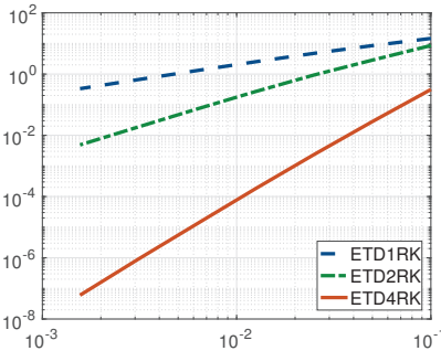
FIG. 4.4. Logarithmic plot of energy errors v.s. time step sizes of the stabilized ETD1RK, ETD2RK, and ETD4RK schemes for the gradient-flow dynamics of two parallel plates with (q_1, q_2) = (0.2e, 0.2e) .
