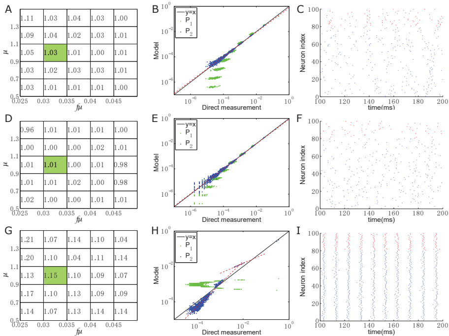
FIG. 7.1. Linearity index and MaxEnt model performance in different dynamical regimes of HH neuronal networks. The network consists of 100 HH neurons (80 Excitatory and 20 Inhibitory) driven by Poisson inputs. The underlying coupling structure for the first row (A-C) is described by a band adjacency matrix, i.e., each neuron is connected to its neighboring 20 postsynaptic neurons. For the second and the third rows (D-I), these are networks with random connections with connection probability 0.2. The coupling strength is selected at random from the uniform distribution of the interval [0, s] , where s = 0.0714 \text{ms}^{-1} for (A-F) and s = 0.429 \text{ms}^{-1} for (G-I) (The corresponding physiological excitatory/inhibitory postsynaptic potential is \sim 1 \text{mV} and \sim 6 \text{mV} for s = 0.0714 \text{ms}^{-1} and 0.429 \text{ms}^{-1} , respectively.). The scanning parameters produce a network with firing rates 3Hz–50Hz for (A-F) and 30Hz–50Hz for (G-I). 10 neurons are selected at random to perform the MaxEnt model analysis. The sampling time bin size is selected to be 10ms. The total recording time is 2 \times 10^4 \text{s} . (A, D, G) The number in each box is the mean value of the linearity index R_T [Equation (6.9)] of all subsets excluding neuron 1 with size N(T) = 2 for a given parameter pair of \mu (ordinate) and f\mu (abscissa) at the lower left corner of each box. For A and D, the standard deviation of R_T for each input is less than 0.03, except for the input of f\mu = 0.025 and f\mu = 0.03 with \mu = 1.3 (The left two boxes of the first row in A and D), where their standard deviations of R_T are less than 0.08 and their corresponding firing rates are less than 5Hz. (B, E, H) For the inputs of the green boxes in the left column (A, D, G), the corresponding rate of occurrence of each firing state predicted from the MaxEnt model distribution of the second order P_2 (blue) and the distribution of the first order MaxEnt model P_1 (green) is plotted against the measured occurrence rate generated from the numerical simulation. We perform the linear fitting in the log-log plot for data points in (B), (E) and (H). The slopes of the linear fitting (dashed red line) are 0.97 and 0.98 for (B) and (E), respectively. Since the points of P_2 in (H) have two distinct regions with different slopes, we perform a linear fitting in the log-log plot in both regions. The slope of the linear fitting (dashed red lines) is 0.56 and 1.28 for the upper and lower regions, respectively. (C, F, I) For the inputs of the green boxes in left column (A, D, G), the corresponding raster plot for inhibitory and excitatory neurons in the network is shown by the red and blue dots, respectively.
