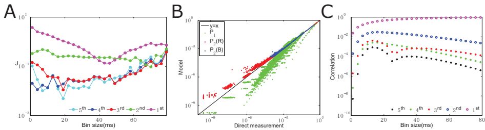
FIG. 8.1. Sensitivity to bin size and dependence on correlations. The simulation is for a network of eight excitatory HH neurons with all-to-all connections. The coupling strength is s = 0.143 \text{ms}^{-1} (The corresponding physiological excitatory postsynaptic potential is \sim 2 \text{mV} ). The input parameters are chosen as \mu = 1 \text{ms}^{-1} and f = 0.035 \text{ms}^{-1} . The mean interspike interval is 42 ms. The total recording time is 1.2 \times 10^7 \text{s} . All 8 neurons are selected to carry out the MaxEnt model analysis. (A) Colored lines correspond to different orders of interactions. The data point is the mean absolute value of interaction strengths of the corresponding order for different sampling time bin sizes, the first order (magenta), the second order (green), the third order (red), the fourth order (blue), and the fifth order (cyan). (B) The rate of occurrence of each firing state predicted from the distribution of the second order MaxEnt model P_2 (The red points are for bin size of 1 ms – 4 ms and 55 ms – 79 ms whereas the blue points are for bin size of 7 ms – 52 ms.) and the distribution of the first order MaxEnt model P_1 (green) is plotted against the measured occurrence rate generated from the numerical simulation. (C) Dots and circles correspond to different orders of correlations. The data point is the mean absolute value of correlation strengths of the corresponding order for different sampling time bin sizes, mean (magenta), the second order (blue), the third order (red), the fourth order (green), and the fifth order (black).
