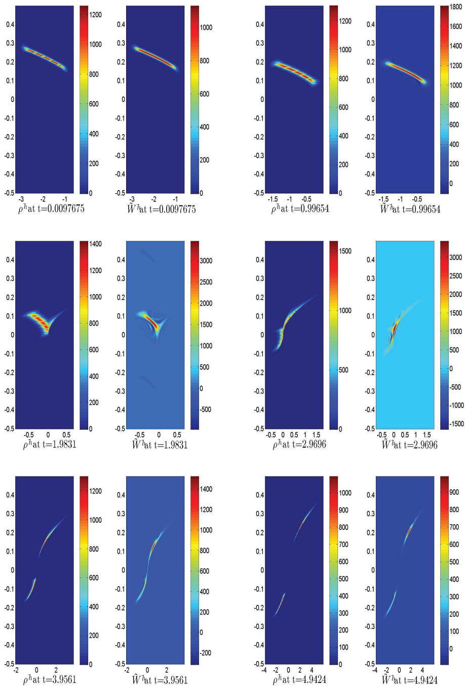
Fig. C.1: The quantum phase-space density \tilde{W}^\varepsilon(t) versus its proposed semiclassical approximation \rho^\varepsilon(t) , for the data of Equation (C.1), \varepsilon = 10^{-2} and various times before, during, and after interaction with the singularity.
