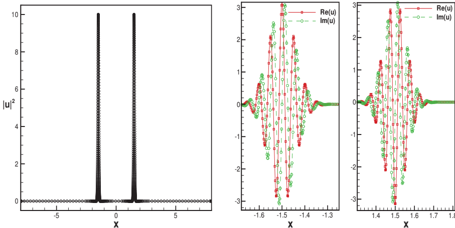
Fig. 6.6: Visualization of u_0 (as defined in Equation (6.8), for \varepsilon = 1e-2 ). Left: Position density. Right: Real and imaginary parts for the two components of u_0 (right).
