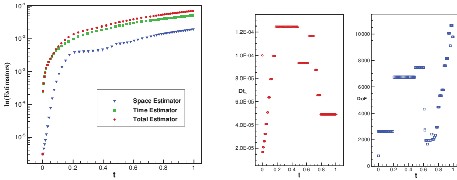
Fig. 5.1: Evolution of estimators in logarithmic scale (left) and variation of the time-steps \Delta t_n and the degrees of freedom (DoF) versus t (right) during adaptivity for V(x,t) = \frac{x^2}{2} \cdot \frac{1}{t+0.05} .
