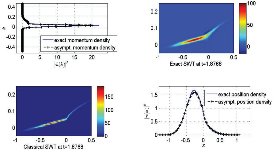
Fig. 6.2: Numerical result for \varepsilon=10^{-2} , m=0.9186 . Top right: Exact SWT. Top left: momentum density ( dx integral of SWT). Bottom right: position density ( dk integral of the SWT). Bottom left: \rho^\varepsilon(t) . (Note that in the SWT plots the wavenumber is scaled with \frac{1}{2\pi} .)
