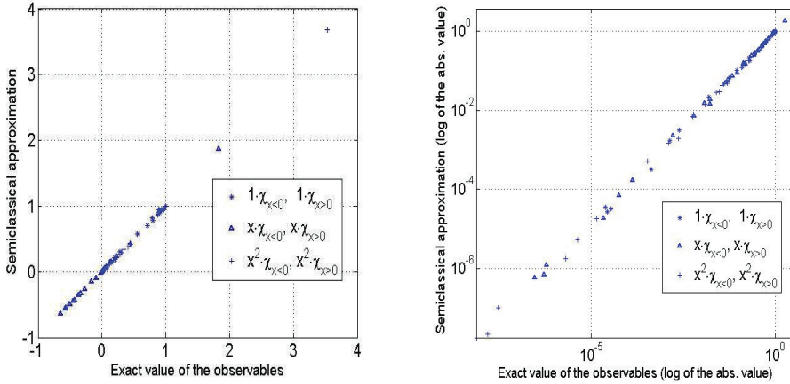
Fig. 6.4: Measurements of observables of position only. The qualitative behavior is consistent with the larger dataset. These benefit from better accuracy, by virtue of Equation (5.12). It is clear that qualitatively the picture doesn't change when we include observables depending on momentum as well (i.e. as in Figure 6.3). This is not surprising, since the simple estimate of Equation (5.13) is known to be pessimistic.
