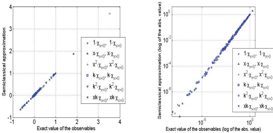
Fig. 6.3: Observable measurements, for the observables in Equation (6.6) and \varepsilon=10^{-2} , m \in \{0.8165, 0.8777, 0.9186, 1.0206, 1.4289\} , at times t \in [1.1788, 2.3577] . The x -coordinate of each point is the measurement on the numerical solution U(t) , \mathcal{A}_{quant} = \langle A(x, k), W^\varepsilon[U(t)] \rangle , and the y -coordinate is the corresponding classical measurement \mathcal{A}_{cl} = \langle A(x, k), P^\varepsilon(t) \rangle . Note that the times used here roughly span the interaction time, in which any discrepancy between the classical and quantum dynamics could occur. More specifically the interaction starts around t=1 and is over by t=2.4 for all the problems.
