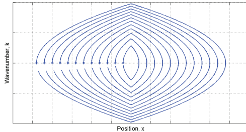
Fig. 3.1: For V=|x| , the characteristics in phase-space can be written explicitly (in each half space \pm X > 0 ) as X(t) = -\frac{1}{2}\text{sign}(X)t^2 + 2\pi K_0 t + X_0 , K(t) = -\frac{1}{2\pi}\text{sign}(X)t + K_0 . Here we see plots of (X(t), K(t)) for various initial conditions (X_0, 0) . All trajectories eventually have corners, but all are uniquely defined. The picture is similar for a \in (0, 1) .
