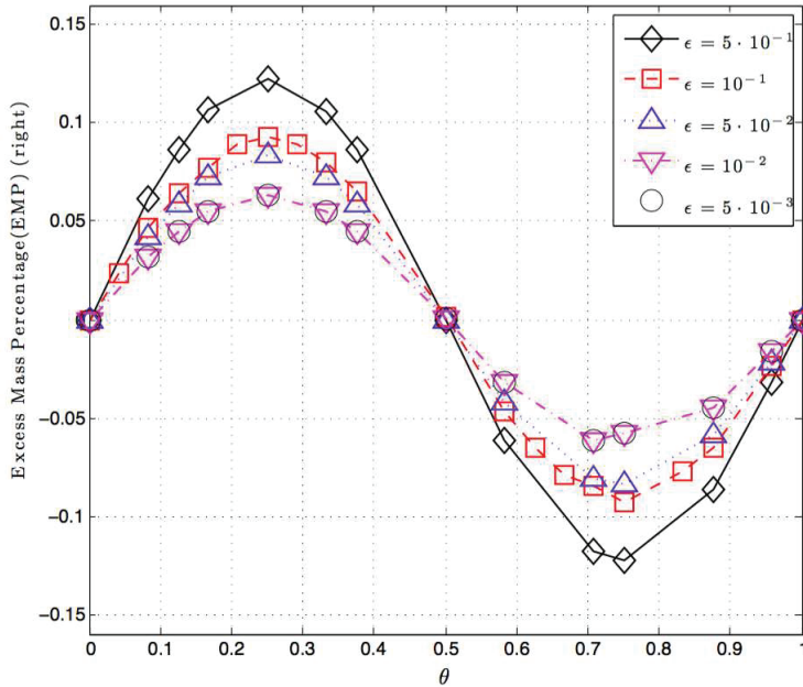
Fig. 6.9: EMP distribution for various values of \theta and \epsilon .
