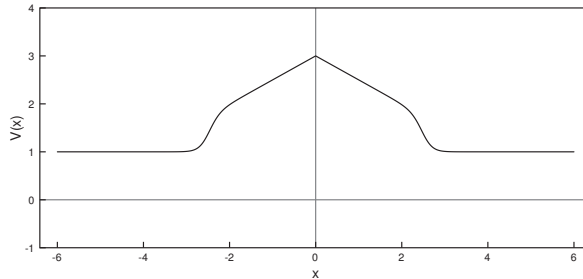
Fig. 6.1: The non-smooth potential V of Equation (6.2).
