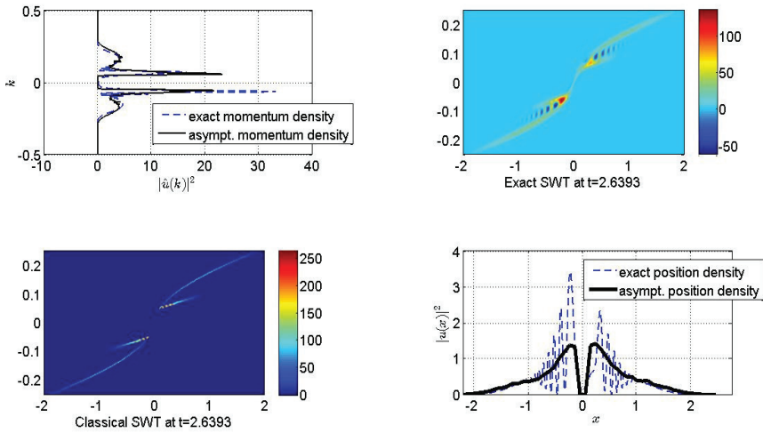
Fig. 6.7: Numerical result for \varepsilon=5 \cdot 10^{-3} , \theta=\frac{18}{24} . Top right: Exact SWT. Top left: momentum density ( dx integral of SWT). Bottom right: position density ( dk integral of the SWT). Bottom left: \rho^\varepsilon(t) . (Note that in the SWT plots the wavenumber is scaled with \frac{1}{2\pi} .)
