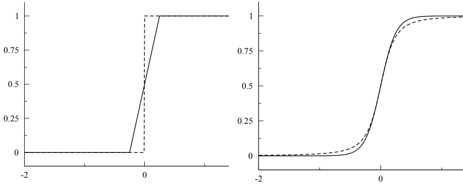
FIG. 2.1. Examples of the liquid fraction functions f and f_\epsilon .
