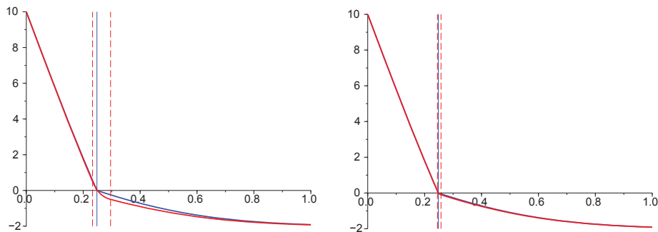
FIG. 5.1. Auto-similar functions u and u_\epsilon with \epsilon = 0.5 (left) and \epsilon = 0.1 (right). T_{(\epsilon)}(x, t) = u_{(\epsilon)}(\frac{x}{\sqrt{t}}) .
