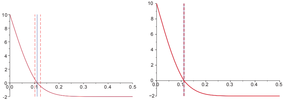
FIG. 5.2. Functions u and u_\epsilon with \epsilon = 0.5 (left) and \epsilon = 0.1 (right).
