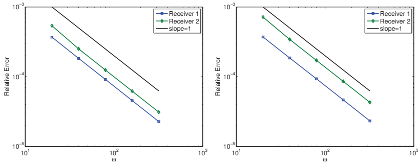
FIG. 6.3. Relative maximum errors by the global geometrical optics approximation.
