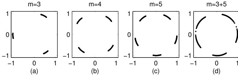
FIG. 7.1. Steady-states arising from custom-designer kernels using 200 particles. (a) Pure mode m=3 instability with g=g^3+1.1158g^0 . (b) Pure mode m=4 instability with g=g^4+1.3g^0 . (c) Pure mode m=5 instability with g=g^5+1.3g^0 . (d) Mixed mode m=3,5 instability with g=1.1225g^3+g^5+1.3g^0 .
