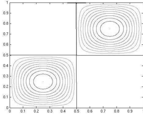
FIG. 3.2. A checkerboard cellular flow.
