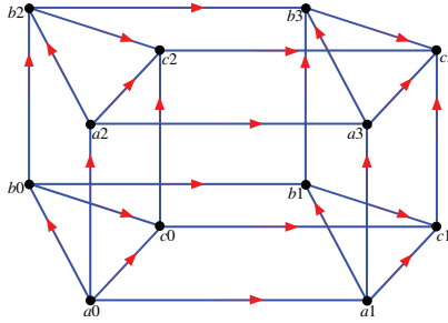
Figure 10: Cartesian product of a triangle and a square.
