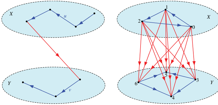
Figure 3: Join of two paths (left) and join of two digraphs (right).
