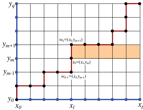
Figure 9: Paths w and z . The shaded area represents L(z) - L(w) .
