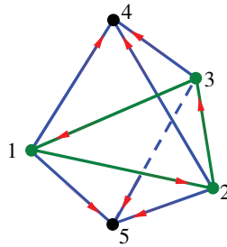
Figure 1: An example of a planar digraph G with non-trivial H_2 .
