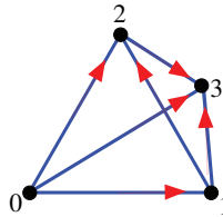
Figure 4: A simplex-digraph \text{Sm}_3 .
