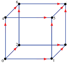
Figure 11: A 3-cube.
