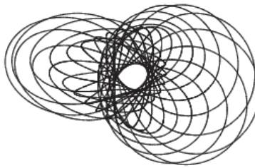
Figure 6: The symmetrical configuration |63, 37, 24 \rangle .
