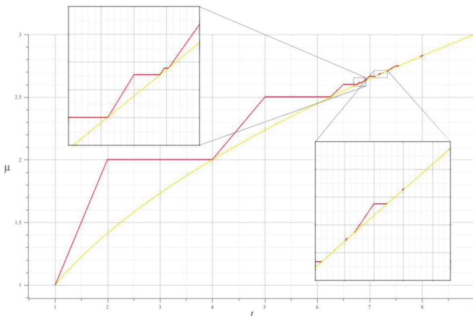
Figure 1: In red, the known behavior of \widehat{\mu}(t) for t \leq 9 ; in yellow, the lower bound \sqrt{t} .
