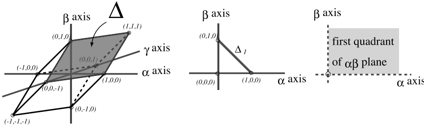
Figure 5: (left) Fiber face \Delta . (center) \Delta_1 \subset \Delta . (right) C_{\Delta_1} \subset \text{int}(C_\Delta) .
