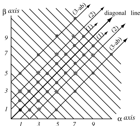
Figure 7: The first quadrant of \alpha\beta plane. Homology classes in (1) (resp. (2), (3a, 3b) of Proposition 3.5) lie on the lines \xrightarrow{(1)} (resp. \xrightarrow{(2)} and \xrightarrow{(3-ab)} ).
