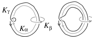
Figure 6: (left) \mathcal{C}_3 . (right) \bar{b} . (this figure explains how to obtain H ).
