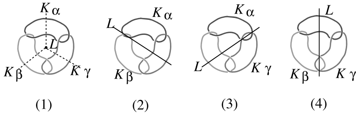
Figure 3: Axis L for periodic map.
