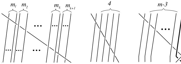
Figure 22: (left) \beta_{(m_1, m_2, \dots, m_{k+1})} . (center) \beta_{(1,4)} . (right) \widehat{\beta}_{(1, m-3)} .
