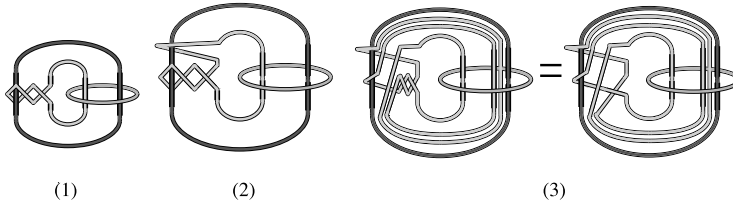
Figure 12: Fiber F_{4,2} with monodromy T_{4,2} associated to (1, 1) . (2) and (3) Describe the first and second part of Case 1 (even), respectively.
