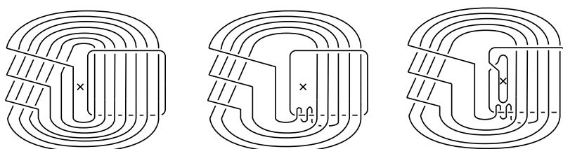
Figure 15: (left) Braided link \bar{b} . (center) Closed 6-braid representing \bar{b} . (right) Closed 7-braid \hat{b}' representing \bar{b} .
