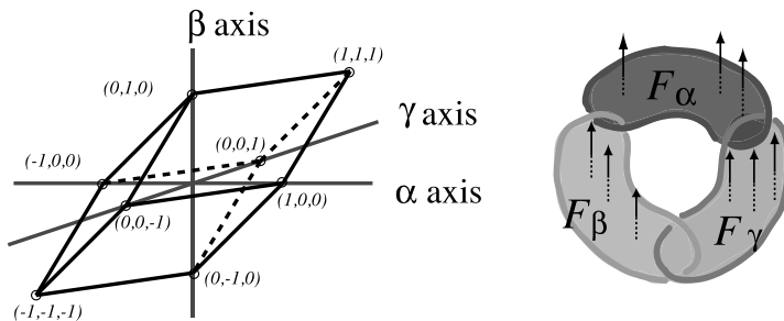
Figure 4: (left) Thurston unit ball. (right) F_\alpha, F_\beta, F_\gamma . (arrows indicate the normal direction of oriented surfaces).
