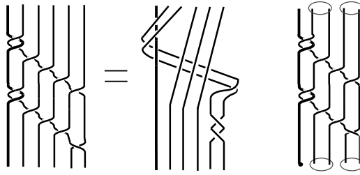
Figure 8: (left) Braid T_{6,2} . (right) Braid T_{5,2} .
