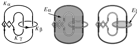
Figure 11: (left) \mathcal{C}_3 . (center), (right) E_\alpha, E_\beta \hookrightarrow E(\mathcal{C}_3) .
