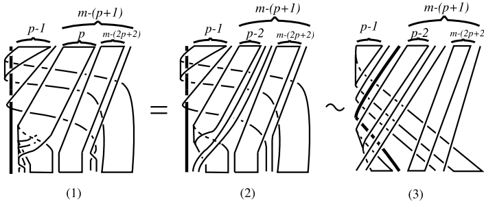
Figure 20: Conjugate braid of T_{m,p} .
