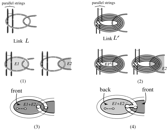
Figure 9: (1) E_1, E_2 \hookrightarrow E(L) . (2) E'_1, E'_2 \hookrightarrow E(L') (in case N = 2 in Lemma 3.12). (3) and (4) E_1 + E_2 \hookrightarrow E(L) .
