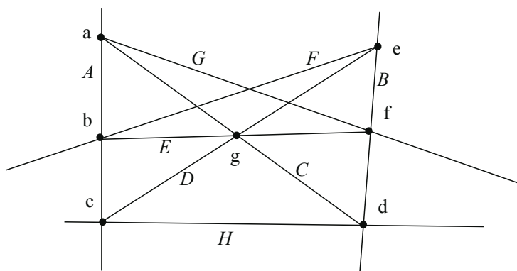
Figure 6: The geometric picture of blowing-up a, b, c, d, e, f, g of the configuration in Table 5.
