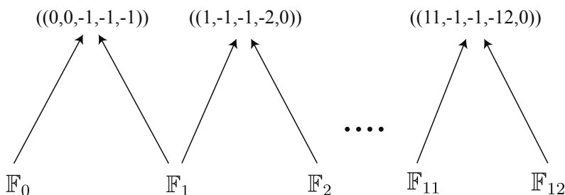
Figure 2: Blowing up Hirzebruch surfaces. For each surface \mathbb{F}_{n \geq 0} , there are only two different ways to blow up it: blow up on the curve of negative self-intersection or blow up at a generic point. For \mathbb{F}_{12} , the (-12) -curve cannot be blown up, as the base of an elliptically fibered Calabi-Yau threefold is not allowed to have curves with self-intersection lower than -12 [14]. The results of blowing up are represented as the self-intersections of the (cyclic) sequence of toric divisors in the blown up surface.
