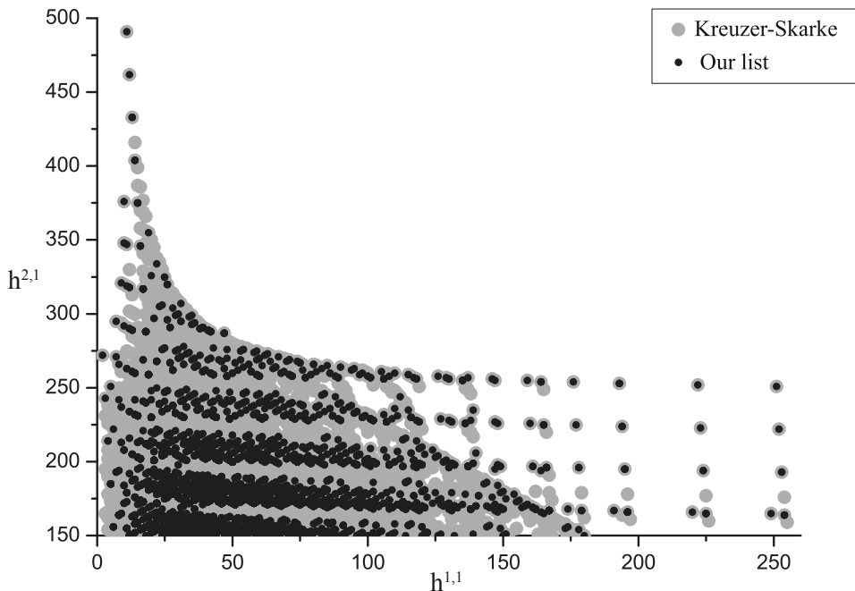
Figure 10: The Hodge numbers of all the EFS Calabi-Yau threefolds with h^{2,1} \geq 150 generated by generic elliptic fibrations over smooth surfaces are represented by black dots. The Hodge numbers in the Kreuzer-Skarke database are represented by gray dots.
