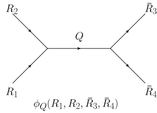
Figure 4: Conformal block \phi_Q(R_1, R_2, \bar{R}_3, \bar{R}_4) for the four-point function.
