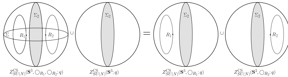
Figure 5: Slicing along \Sigma_2 \simeq \mathbf{S}^2 .
