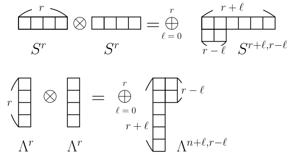
Figure 6: Young diagrams for tensor products of symmetric and anti-symmetric representations.
