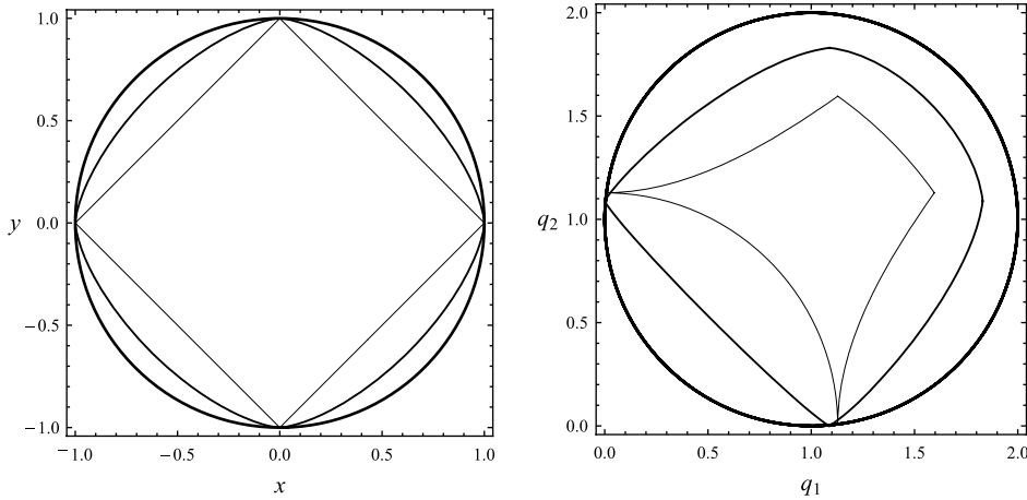
Figure 4: Left: circles in two dimensions with unit radius in 2\alpha -norm, |x|^{2\alpha} + |y|^{2\alpha} = 1 ; increasing thickness corresponds to \alpha = 1/2, 3/4, 1 . Right: the same circles in left geometric coordinates q_1 = (x - x_0)^\alpha / \Gamma(\alpha + 1) and q_2 = (y - y_0)^\alpha / \Gamma(\alpha + 1) , with x_0 = -1 = y_0 .
