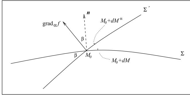
Figure 2: Geometric interpretation of fractional gradient. The symbols are explained in the text.
