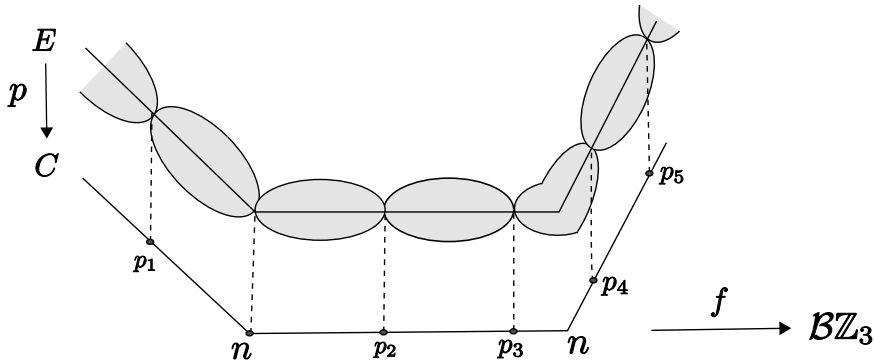
Figure 1: A map C \rightarrow \mathcal{B}\mathbb{Z}_3 corresponds to an admissible cover of C . Notice that not all marked points must be twisted.
