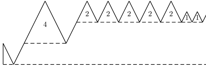
Figure 4: Minimal path corresponding to the path of figure 3 with k = 6 . All particles are moved to the right as much as possible and arranged in decreasing order with respect to charge such that the maximal height of the path does not exceed k and such that the final step remains upwards.
