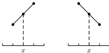
Figure 2: Vertices of weight x .
