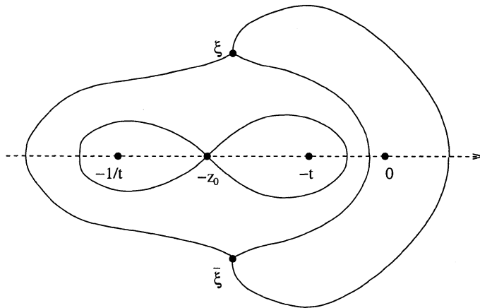
Figure 10: Global structure of the trajectories of Q(dz)^2 .
