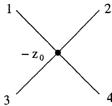
Figure 4: Local structure of the trajectories of Q(dz)^2 near -z_0 .
