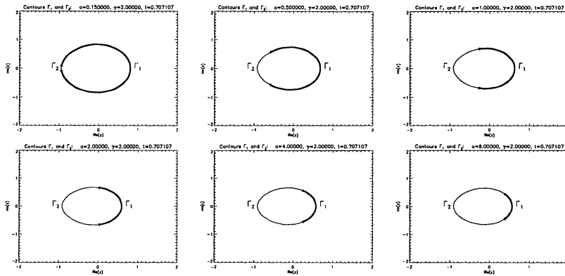
Figure 16: The dependence of the contours \Gamma_1 and \Gamma_2 on the parameter a . As a tends to a_0 from above, the endpoints \xi and \bar{\xi} coalesce on the negative real axis.
