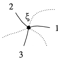
Figure 12: Orthogonal trajectories and trajectories emerging from \xi .
