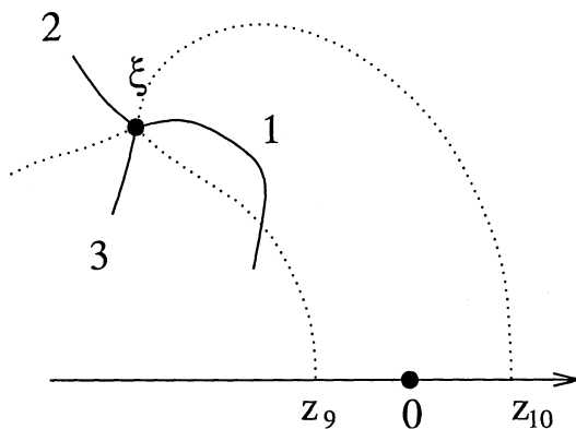
Figure 13: Orthogonal trajectories emerging from \xi .
