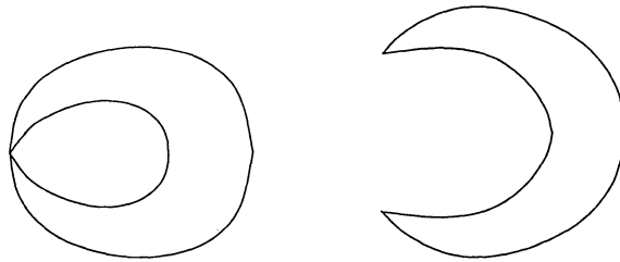
Figure 5: Unfolding of “closed” trajectories meeting at a point.
