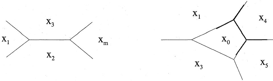
Figure 3: The moment map for the LSM defined by (35) and the projection to x_2 = 0 of the momentum map for the LSM on the 4-fold (40). We have also indicated how the momentum map for the spin bundle \Sigma_{S^3_1} sits in the latter (blue lines).
