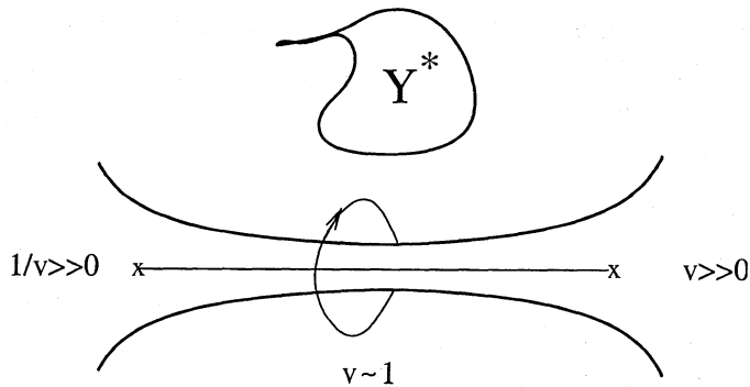
Figure 1: The Calabi–Yau manifold X^* is a “fibration” of Y^* over a cylinder with branch points, in the limit where the cylinder becomes infinitely long.
