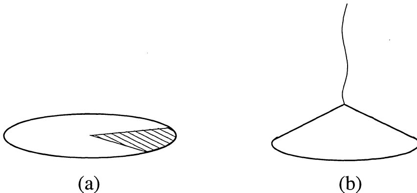
Figure 3: (a) Deficit angle in the intrinsic horizon 2-geometry. (b) A 3-dimensional perspective: a bulk polymer excitation ‘exerts a tug’ on the horizon causing a deficit angle.
