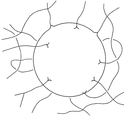
Figure 2: Quantum Horizon. Polymer excitations in the bulk puncture the horizon, endowing it with quantized area. Intrinsically, the horizon is flat except at punctures where it acquires a quantized deficit angle. These angles add up to 4\pi .
