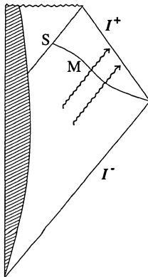
Figure 1: A typical spacetime of interest depicting a gravitational collapse. The horizon geometry becomes time-independent at late times, say to the future of a cross-section S . However, there is gravitational radiation crossing any (partial) Cauchy surface M in the exterior region.
