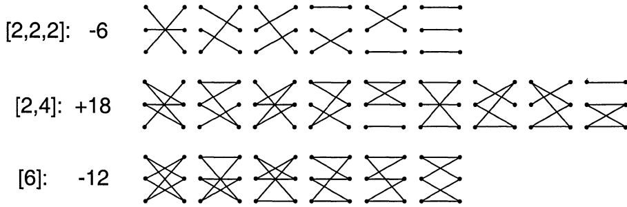
Figure 1: Bipartite graphs relevant for K = 2 . Each point on the left of a diagram corresponds to an operator (k \cdot \psi)\Psi , while on the right it correspond to (k \cdot \psi)\bar{\Psi} . Each loop has to be counted twice, reflecting the two ways to assign to it an alternating sequence of \psi\bar{\psi} and \Psi\bar{\Psi} propagators. The cycle structure also determines the signs.
