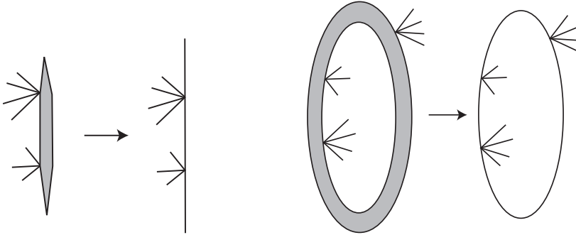
FIG. 6. Two cases in which L_0 collapses to a geodesic
