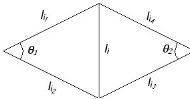
FIG. 1. Edge lengths adjacent to e_i
