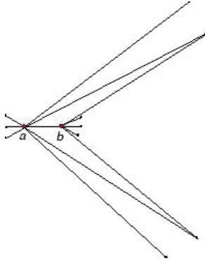
FIG. 7. A configuration which ceases to be embedded under the gradient flow. The vertex a moves rightward faster than vertex b .
