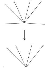
FIG. 4. A vertex limiting to meet the interior of an edge.
