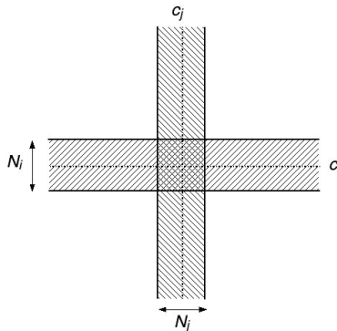
FIG. 3. Intersection of N_i and N_j
