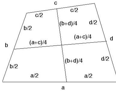
FIG. 2. Conformal subdivision preserves area.
