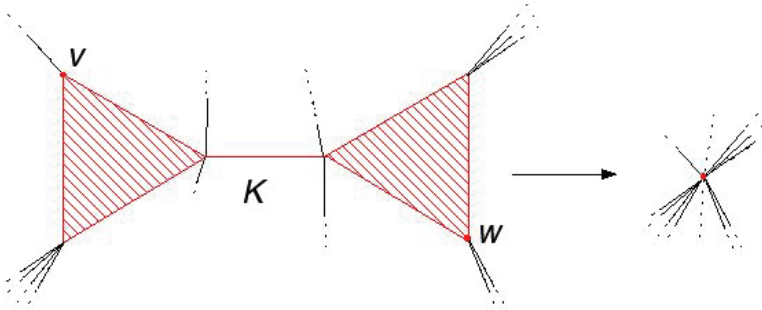
FIG. 5. A subcomplex collapses to a point.
