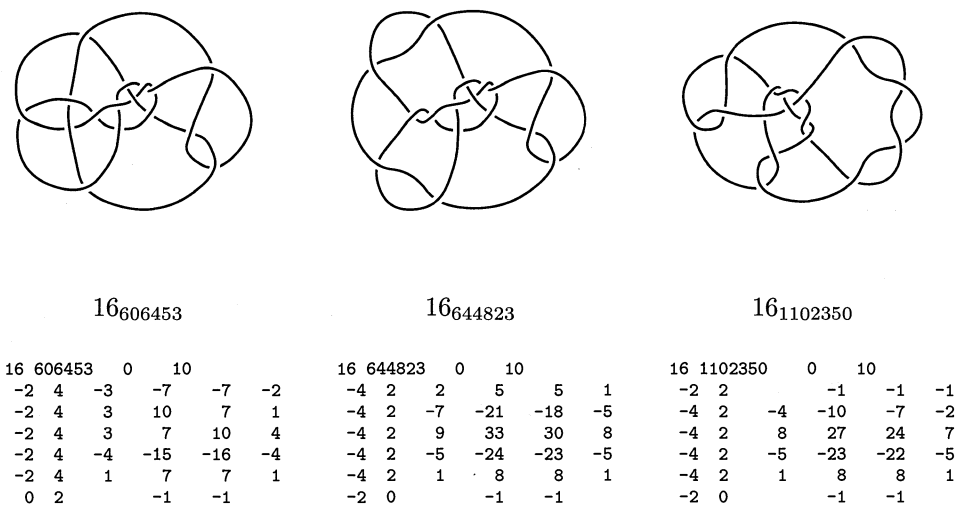
FIG. 1. Three of the examples of Theorem 1.1 and their skein polynomials. All three knots have the Alexander polynomial \Delta = -1\ 4\ -8\ [11]\ -8\ 4\ -1 .
