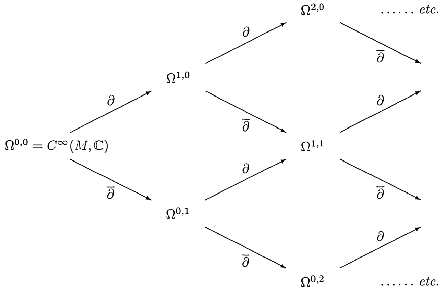
FIG. 3.1. The Dolbeault Complex
