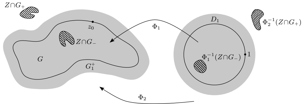
Figure 1. The two conformal mappings \Phi_1 and \Phi_2 , the domain D_1 and the possible location of poles.
